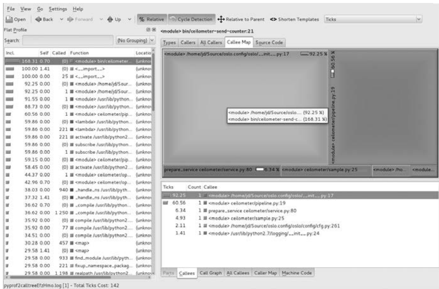
Figure 10-1: Example of KCachegrind output
